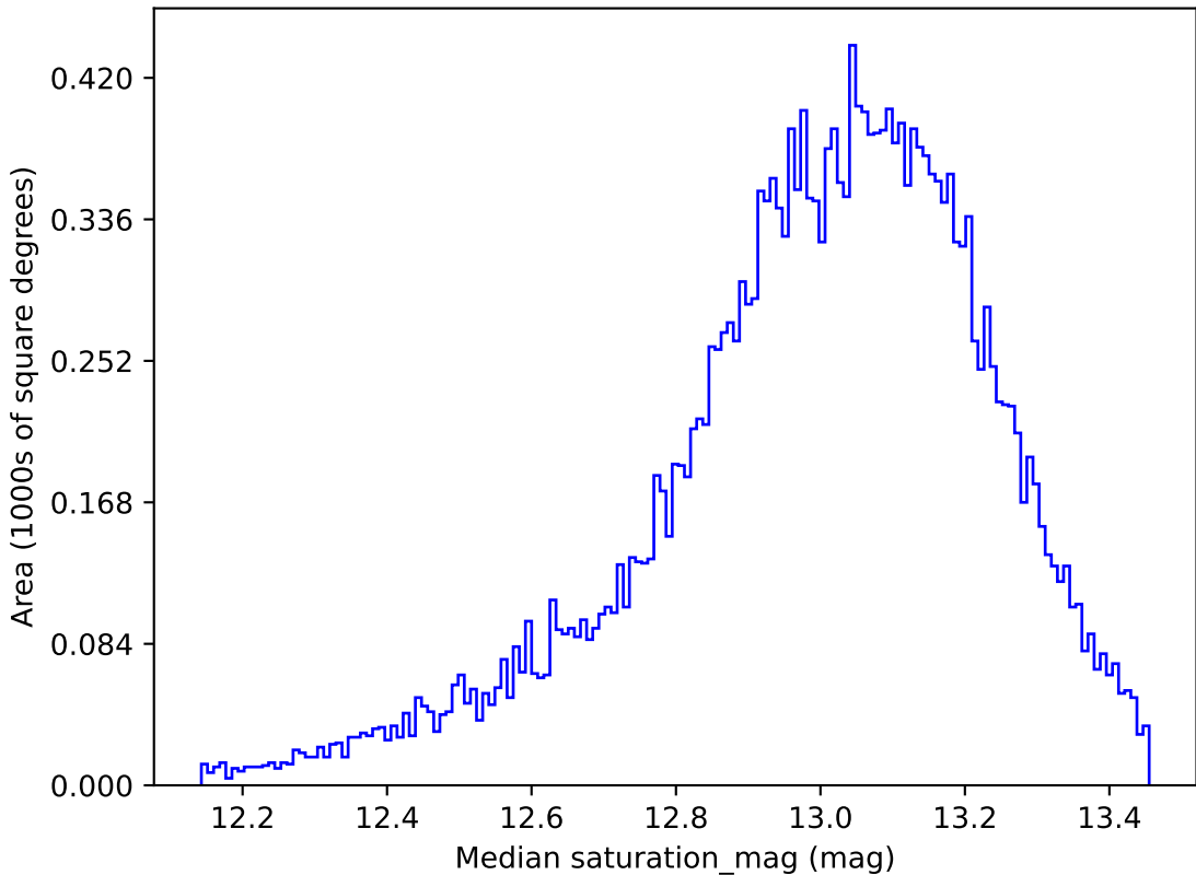
noroll_mjdp60_v3.4_10yrs All sky u band: Median saturation_mag
