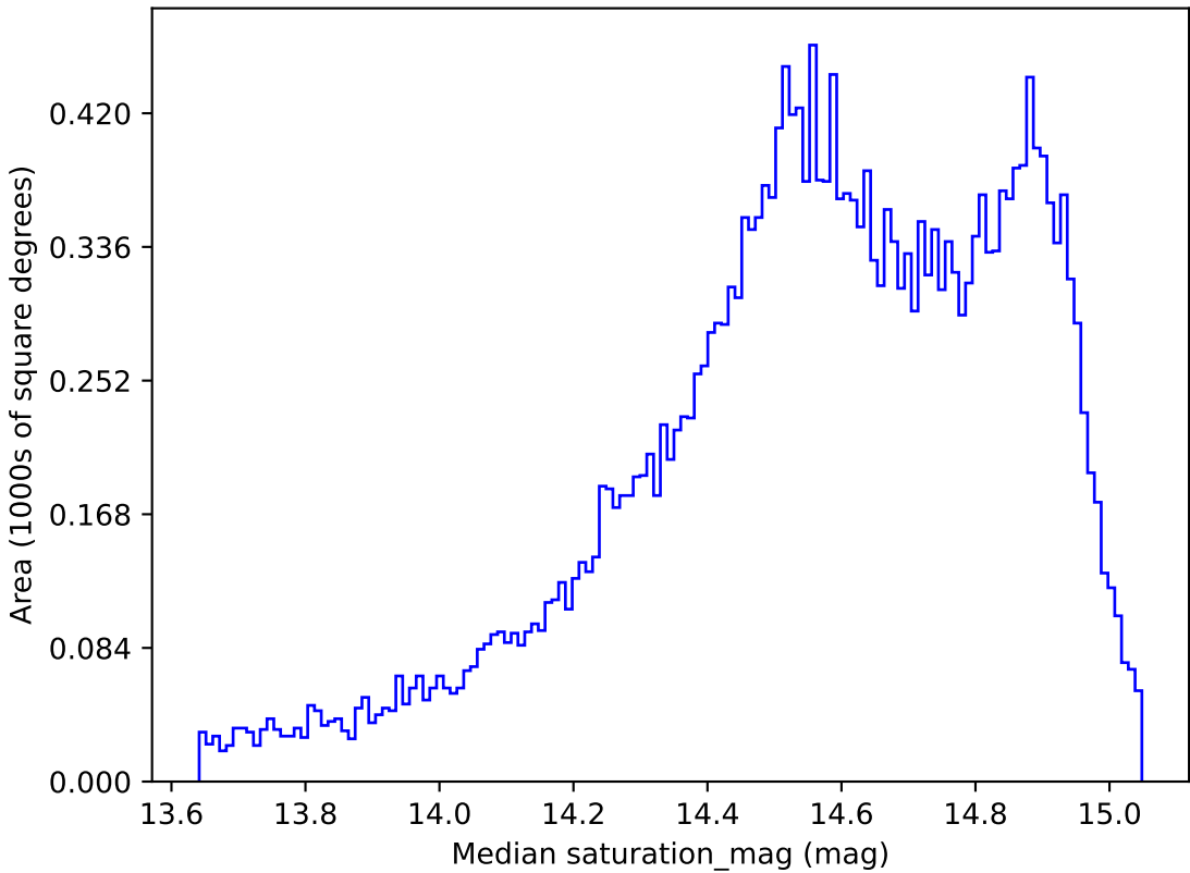
noroll_mjdp60_v3.4_10yrs All sky r band: Median saturation_mag
