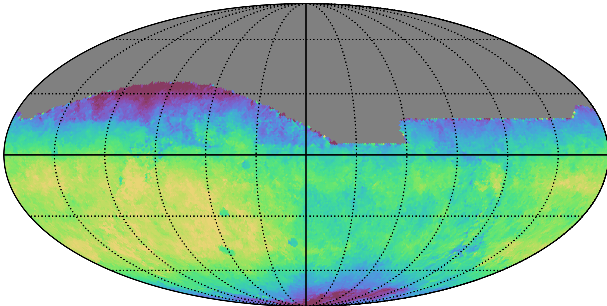
noroll_mjdp60_v3.4_10yrs All sky i band: Median saturation_mag
