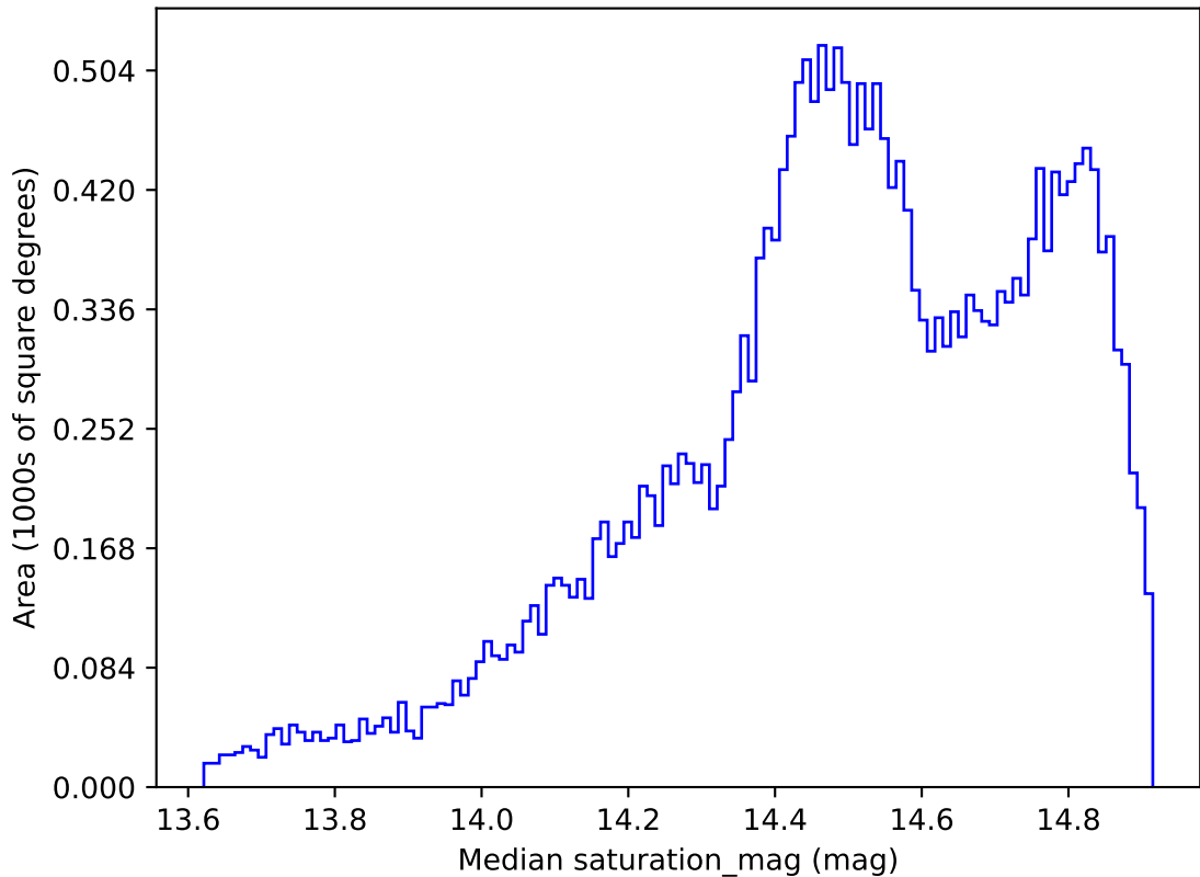
noroll_mjdp60_v3.4_10yrs All sky i band: Median saturation_mag
