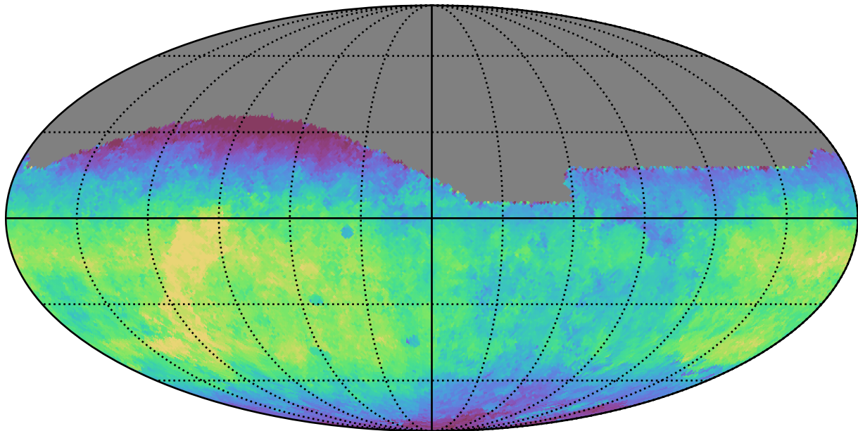
noroll_mjdp60_v3.4_10yrs All sky g band: Median saturation_mag
