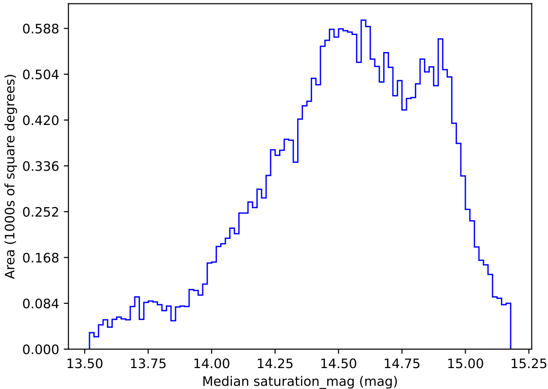
noroll_mjdp60_v3.4_10yrs All sky g band: Median saturation_mag
