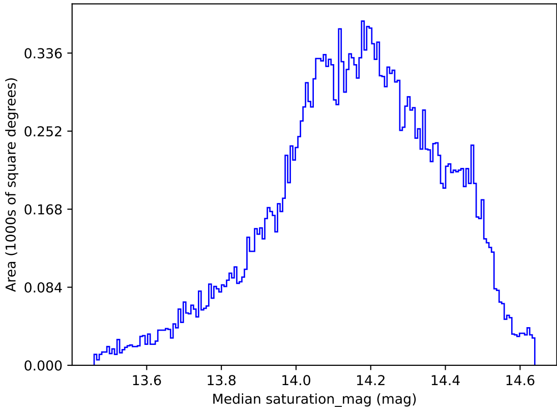
noroll_mjdp60_v3.4_10yrs All sky all bands: Median saturation_mag
