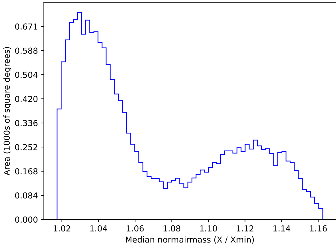
noroll_mjdp60_v3.4_10yrs WFD z band: Median normairmass
