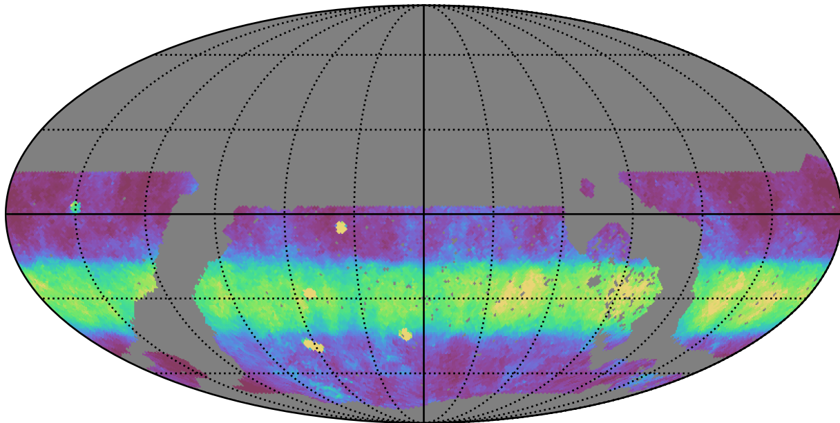
noroll_mjdp60_v3.4_10yrs WFD y band: Median normairmass
