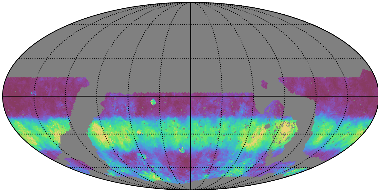
noroll_mjdp60_v3.4_10yrs WFD g band: Median normairmass
