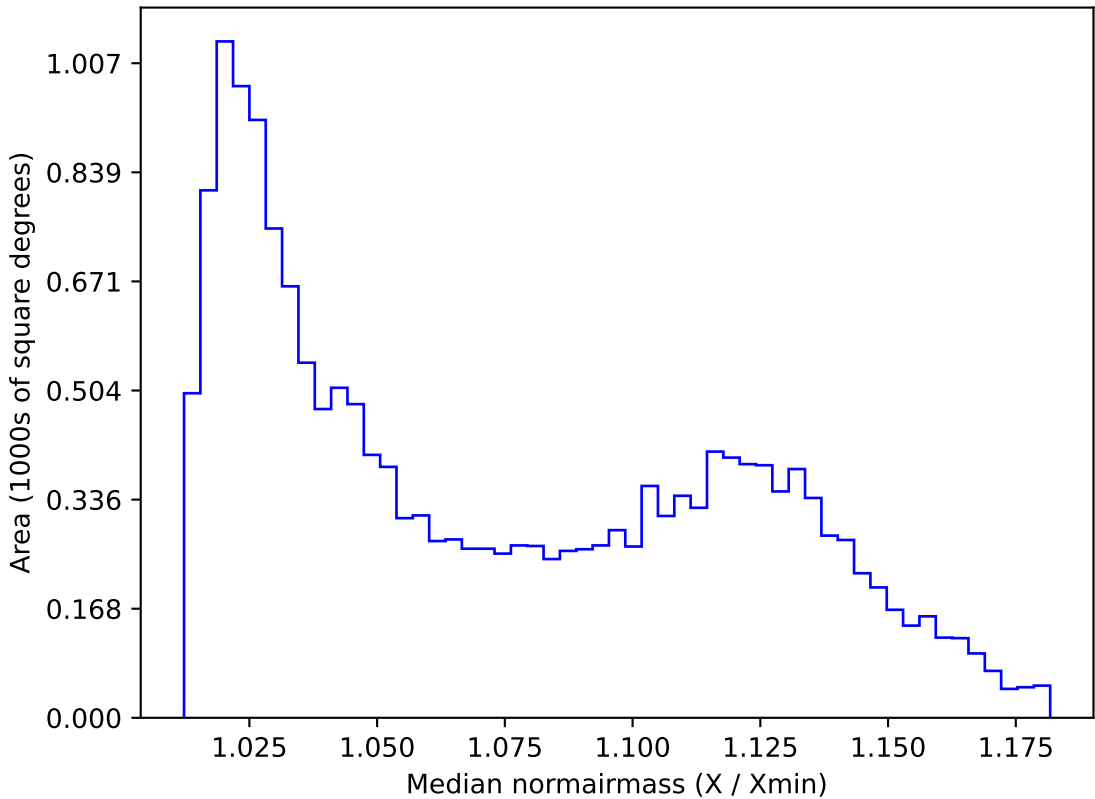
noroll_mjdp60_v3.4_10yrs WFD g band: Median normairmass
