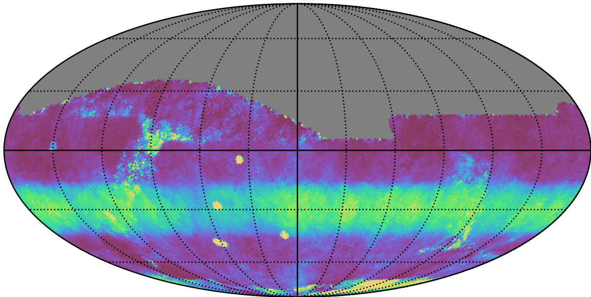
noroll_mjdp60_v3.4_10yrs All sky z band: Median normairmass
