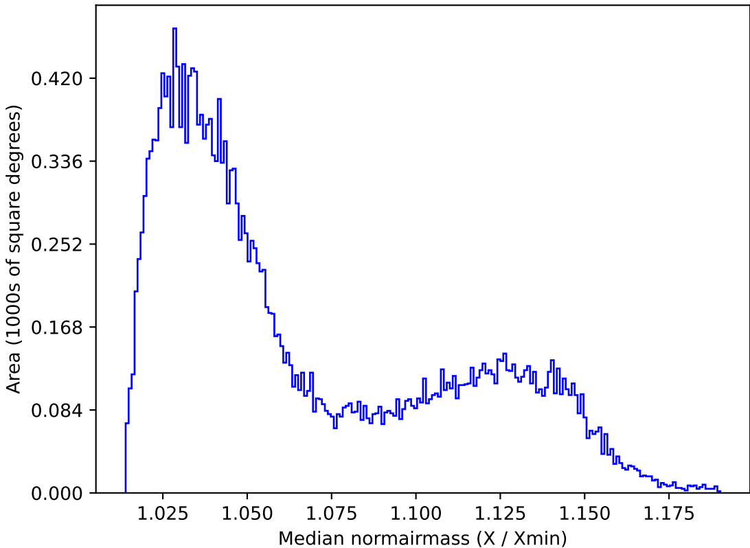
noroll_mjdp60_v3.4_10yrs All sky z band: Median normairmass
