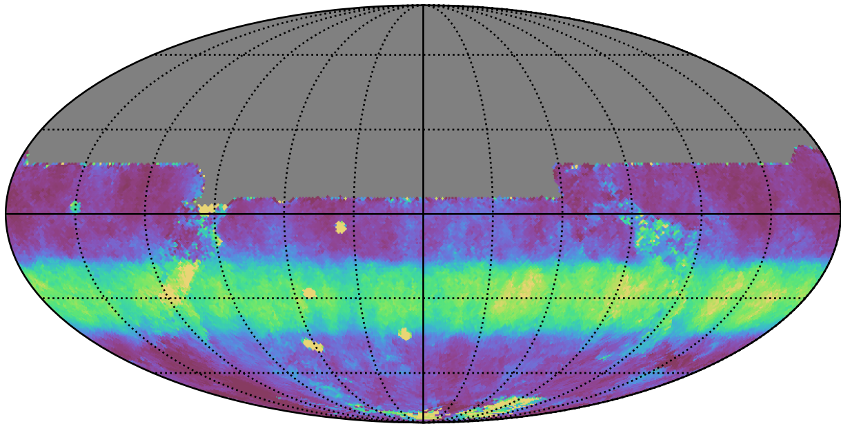
noroll_mjdp60_v3.4_10yrs All sky y band: Median normairmass
