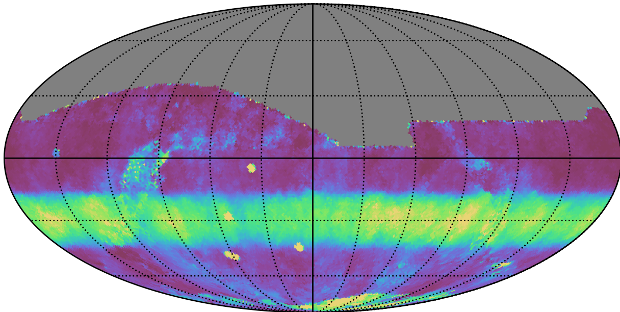
noroll_mjdp60_v3.4_10yrs All sky r band: Median normairmass
