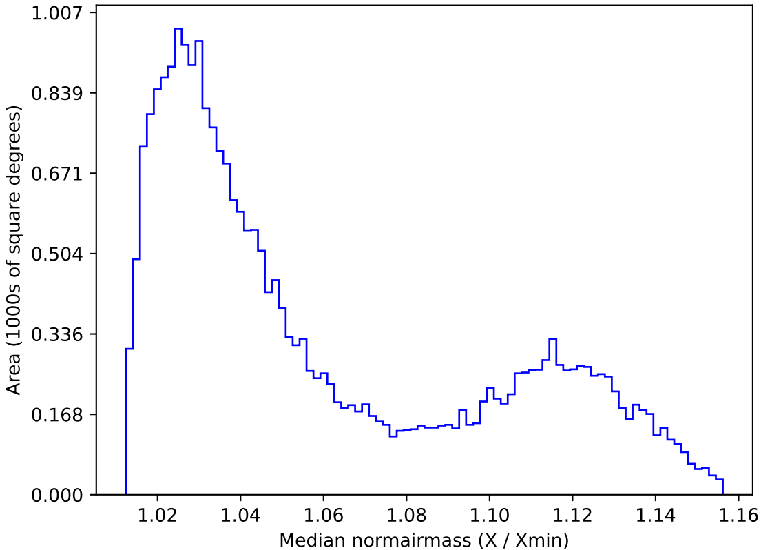
noroll_mjdp60_v3.4_10yrs All sky r band: Median normairmass
