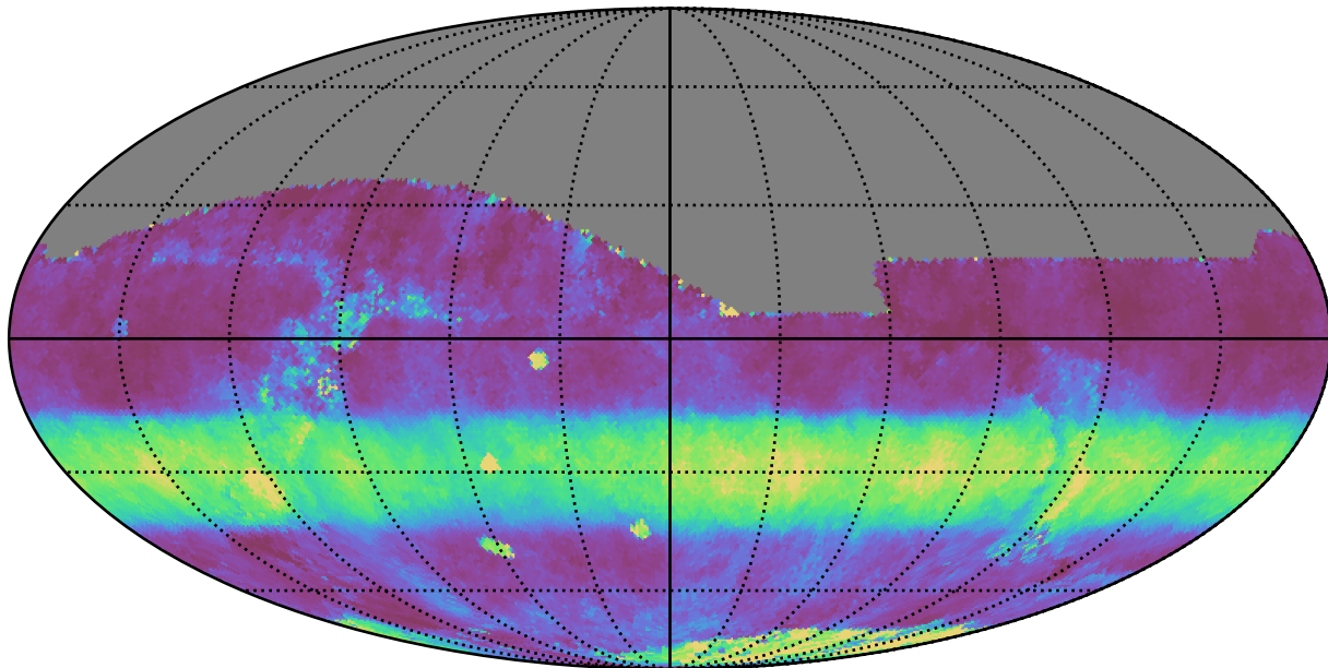
noroll_mjdp60_v3.4_10yrs All sky i band: Median normairmass
