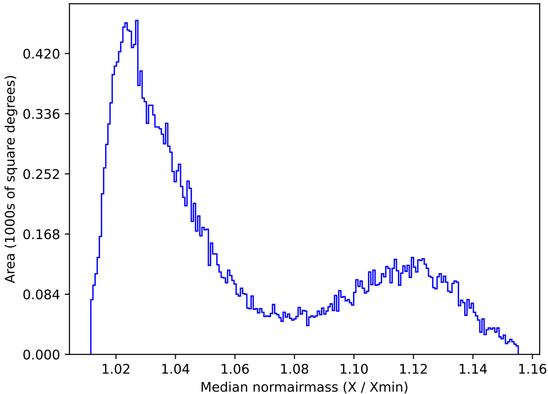
noroll_mjdp60_v3.4_10yrs All sky i band: Median normairmass
