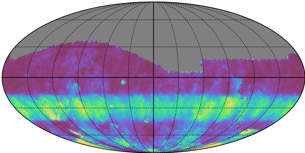
noroll_mjdp60_v3.4_10yrs All sky g band: Median normairmass
