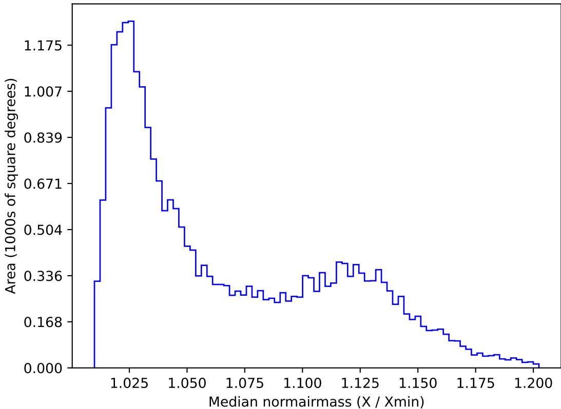
noroll_mjdp60_v3.4_10yrs All sky g band: Median normairmass
