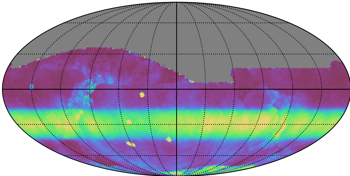
noroll_mjdp60_v3.4_10yrs All sky all bands: Median normairmass
