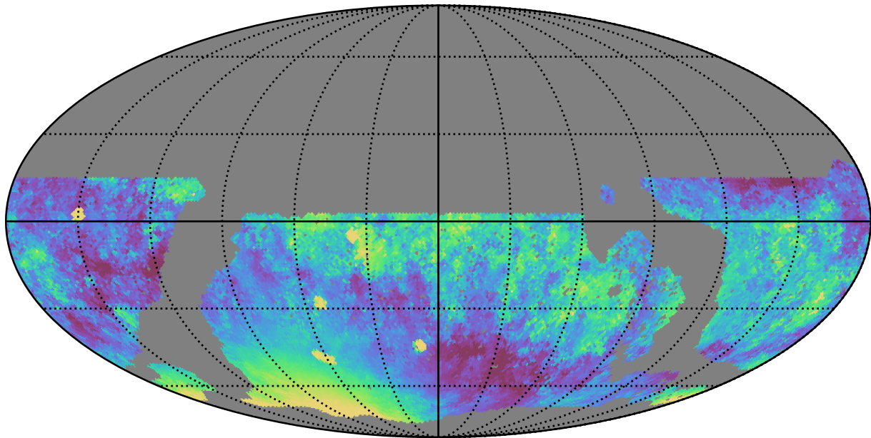
noroll_mjdp60_v3.4_10yrs WFD z band: Median moonDistance
