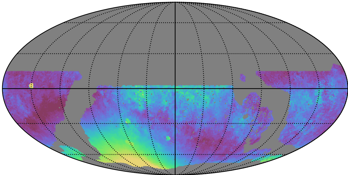
noroll_mjdp60_v3.4_10yrs WFD y band: Median moonDistance
