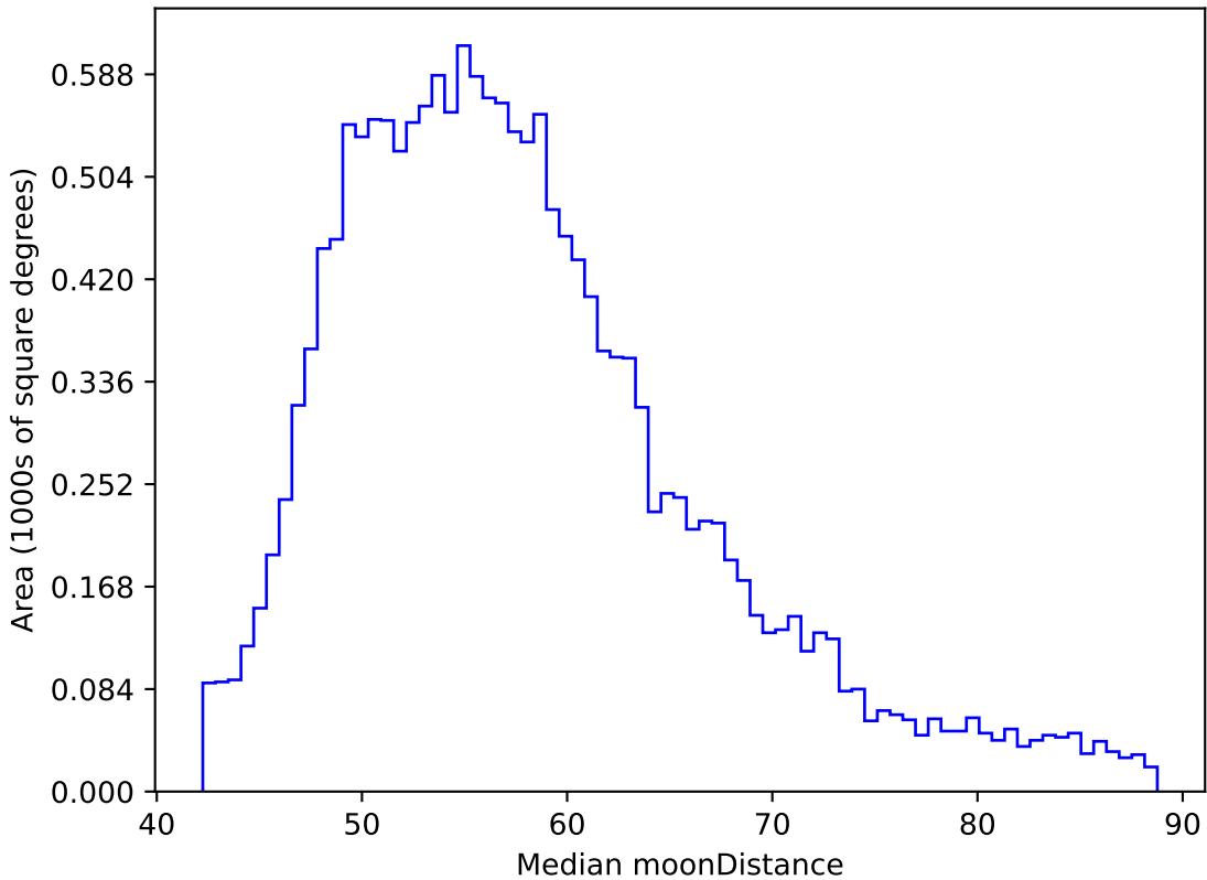
noroll_mjdp60_v3.4_10yrs WFD y band: Median moonDistance
