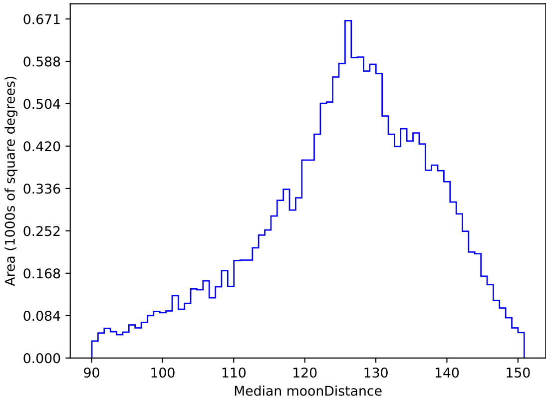
noroll_mjdp60_v3.4_10yrs WFD u band: Median moonDistance
