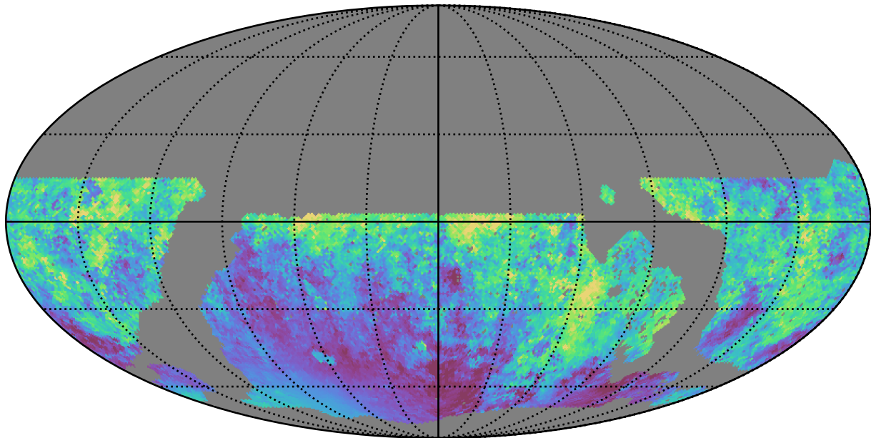
noroll_mjdp60_v3.4_10yrs WFD i band: Median moonDistance
