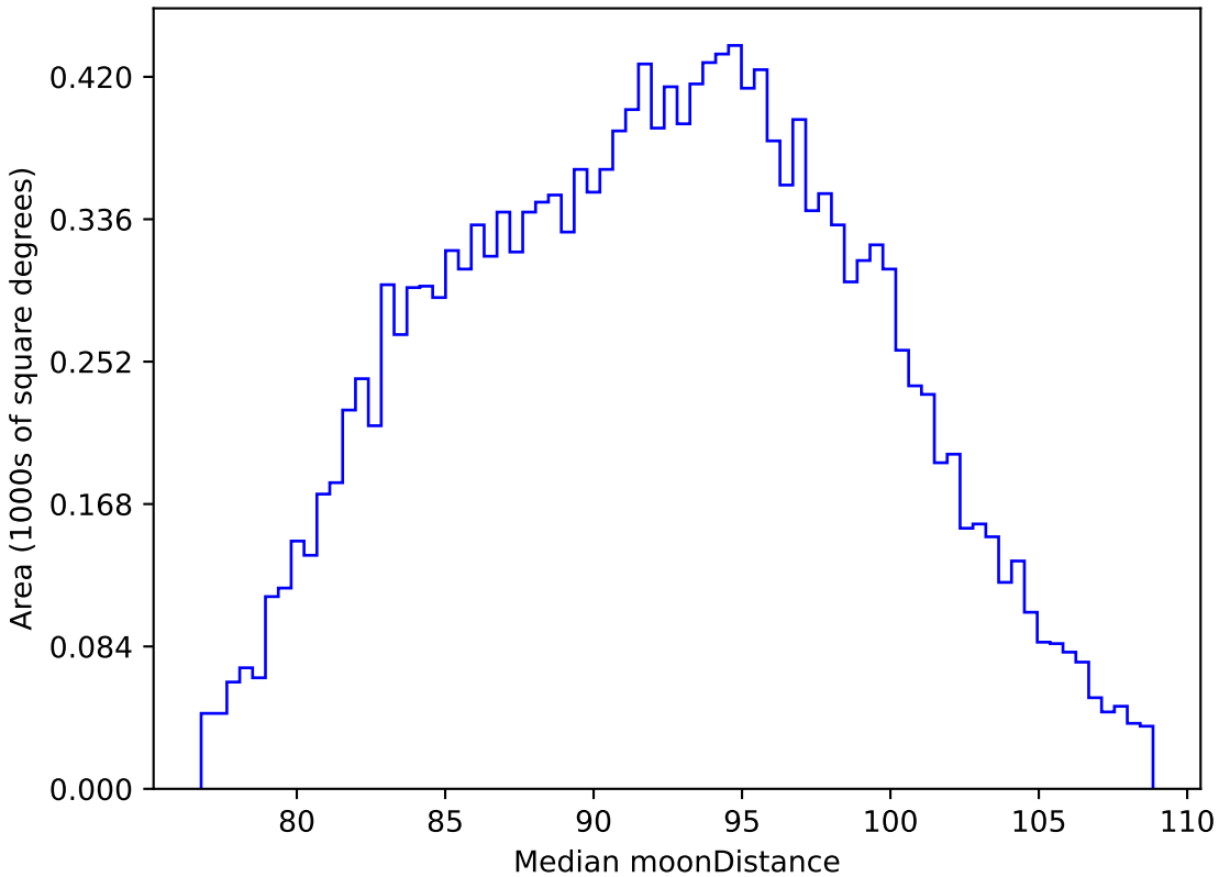
noroll_mjdp60_v3.4_10yrs WFD i band: Median moonDistance
