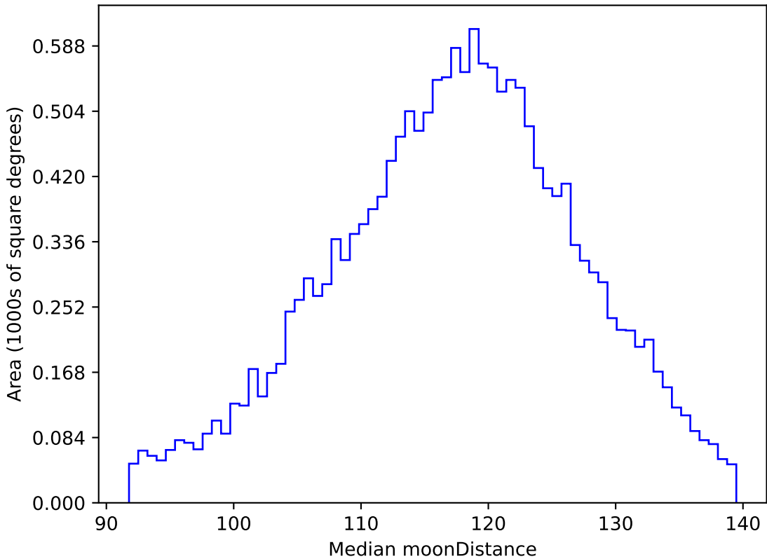
noroll_mjdp60_v3.4_10yrs WFD g band: Median moonDistance
