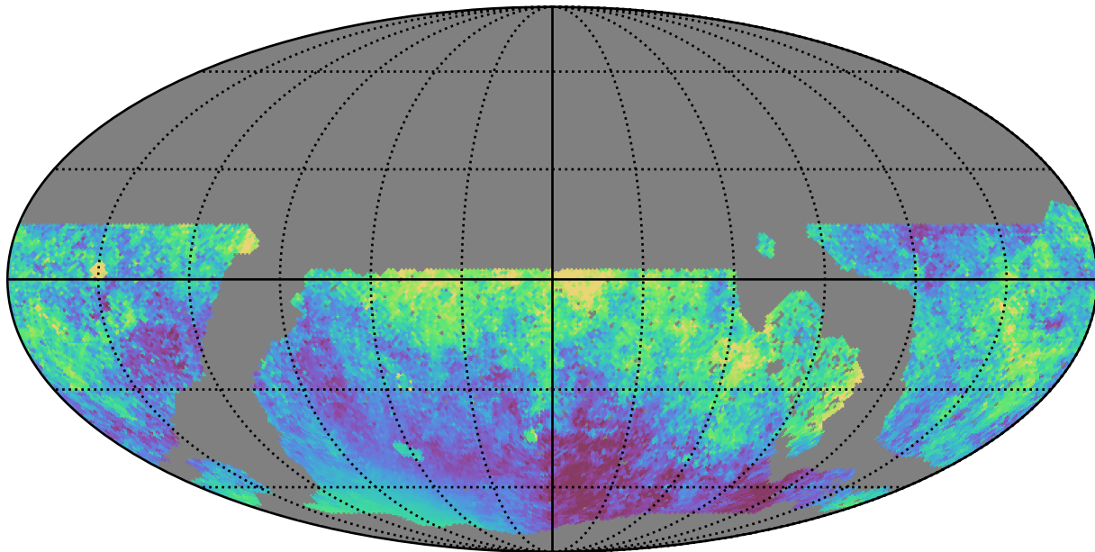
noroll_mjdp60_v3.4_10yrs WFD all bands: Median moonDistance
