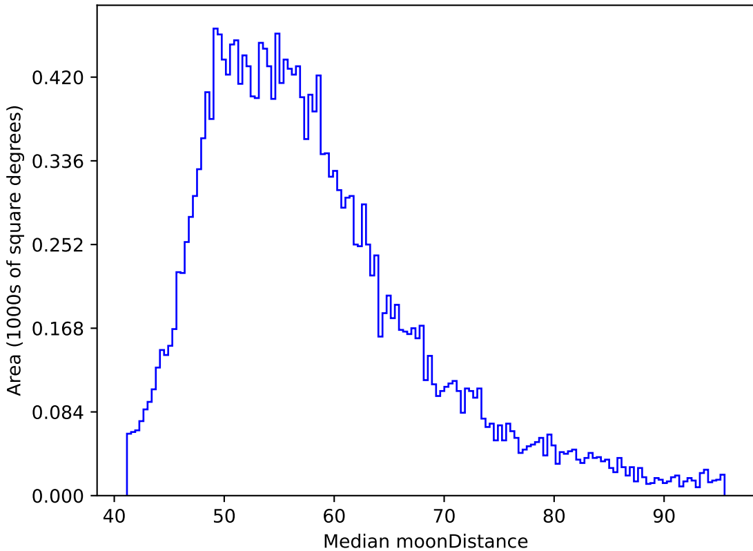
noroll_mjdp60_v3.4_10yrs All sky y band: Median moonDistance
