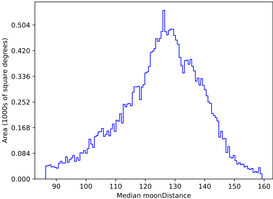
noroll_mjdp60_v3.4_10yrs All sky u band: Median moonDistance
