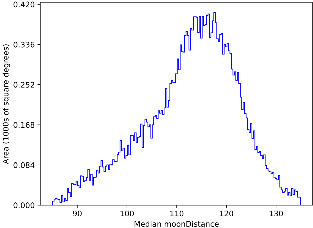
noroll_mjdp60_v3.4_10yrs All sky r band: Median moonDistance
