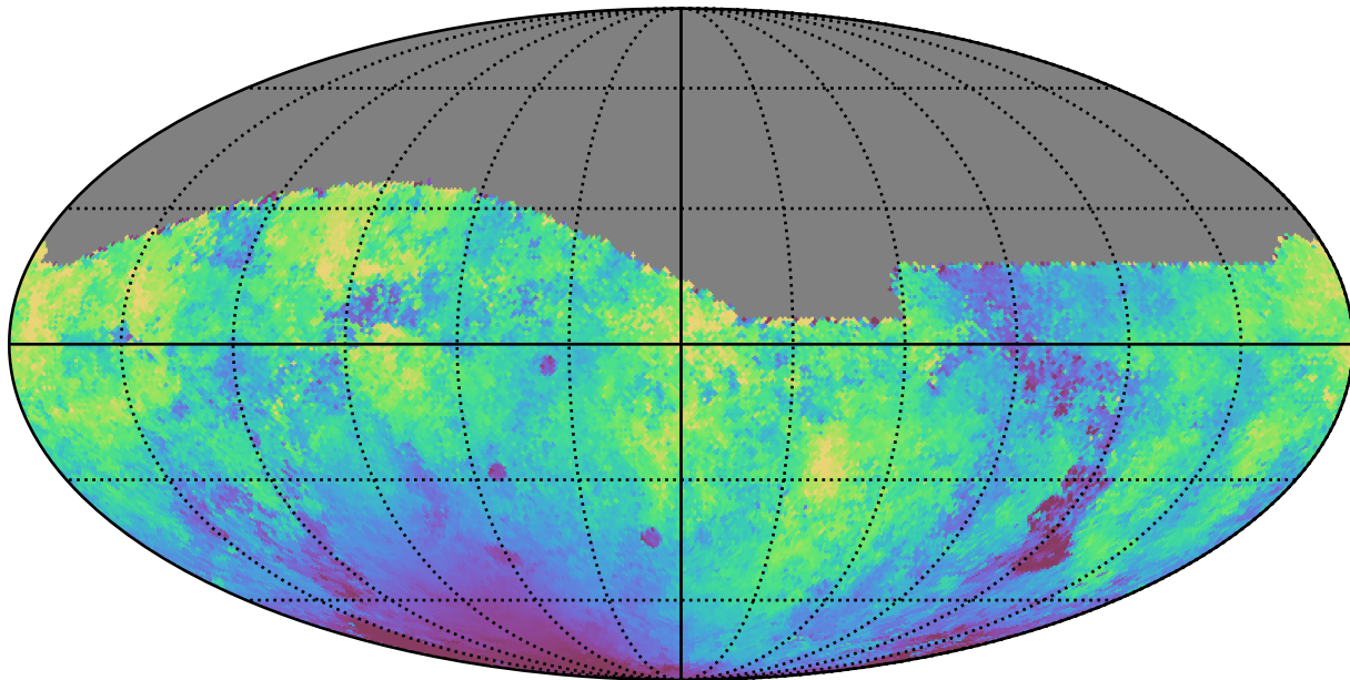
noroll_mjdp60_v3.4_10yrs All sky g band: Median moonDistance
