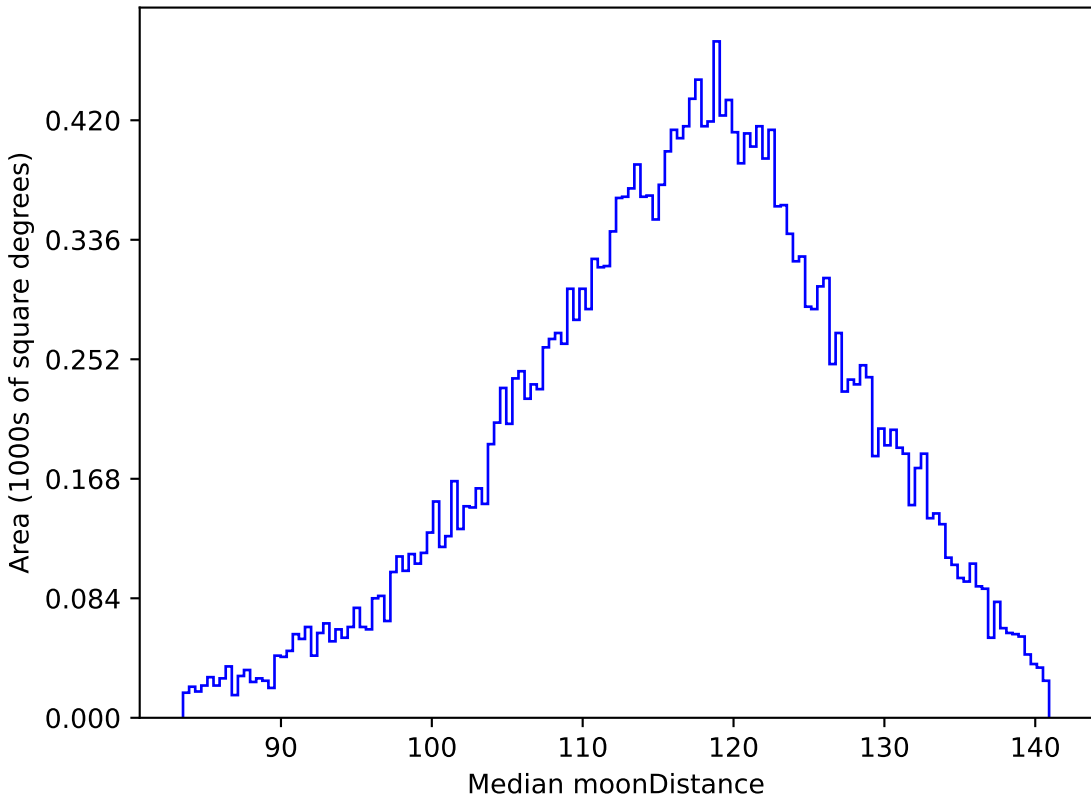
noroll_mjdp60_v3.4_10yrs All sky g band: Median moonDistance
