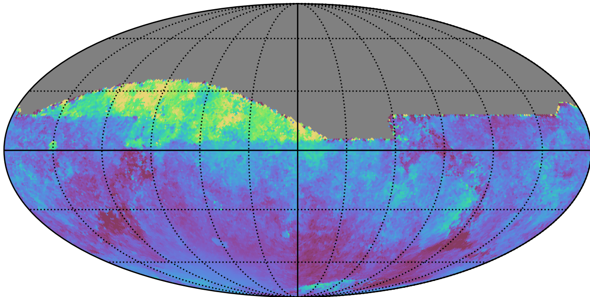
noroll_mjdp60_v3.4_10yrs All sky all bands: Median moonDistance
