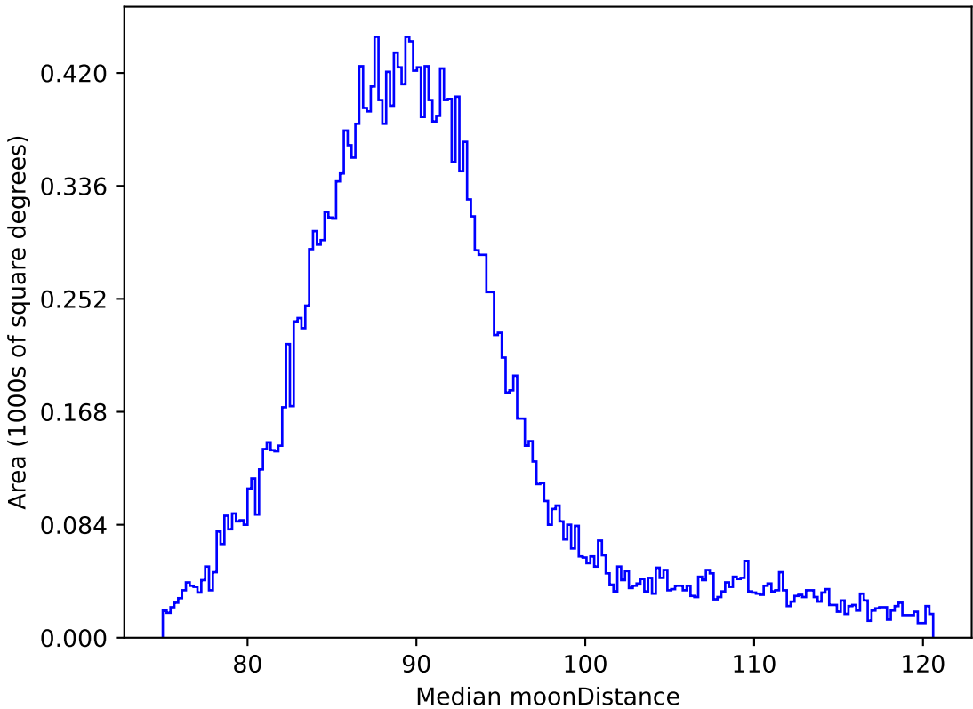
noroll_mjdp60_v3.4_10yrs All sky all bands: Median moonDistance
