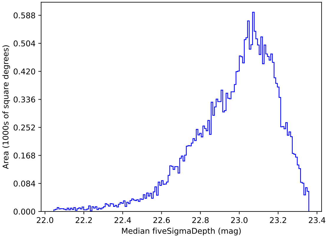
noroll_mjdp60_v3.4_10yrs Yr 1 z band: Median fiveSigmaDepth
