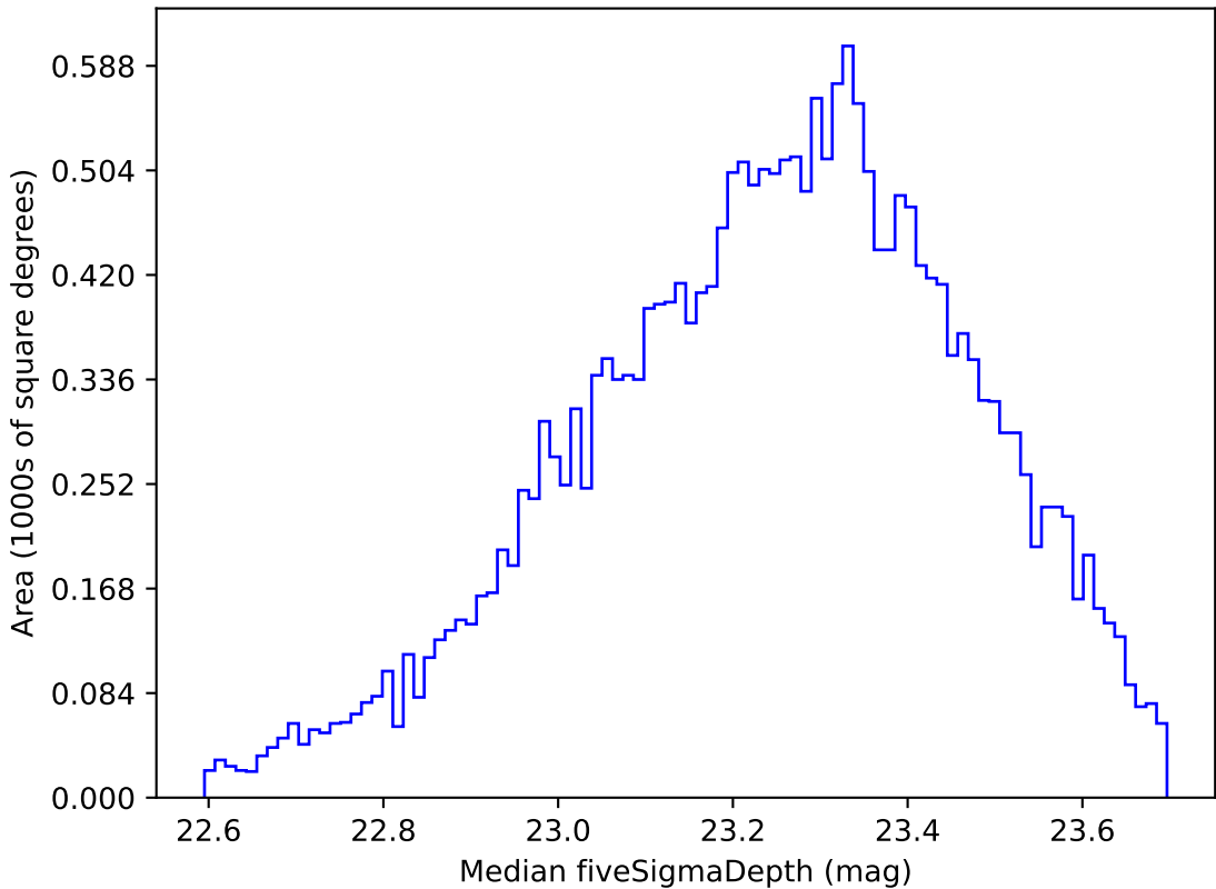
noroll_mjdp60_v3.4_10yrs Yr 1 u band: Median fiveSigmaDepth
