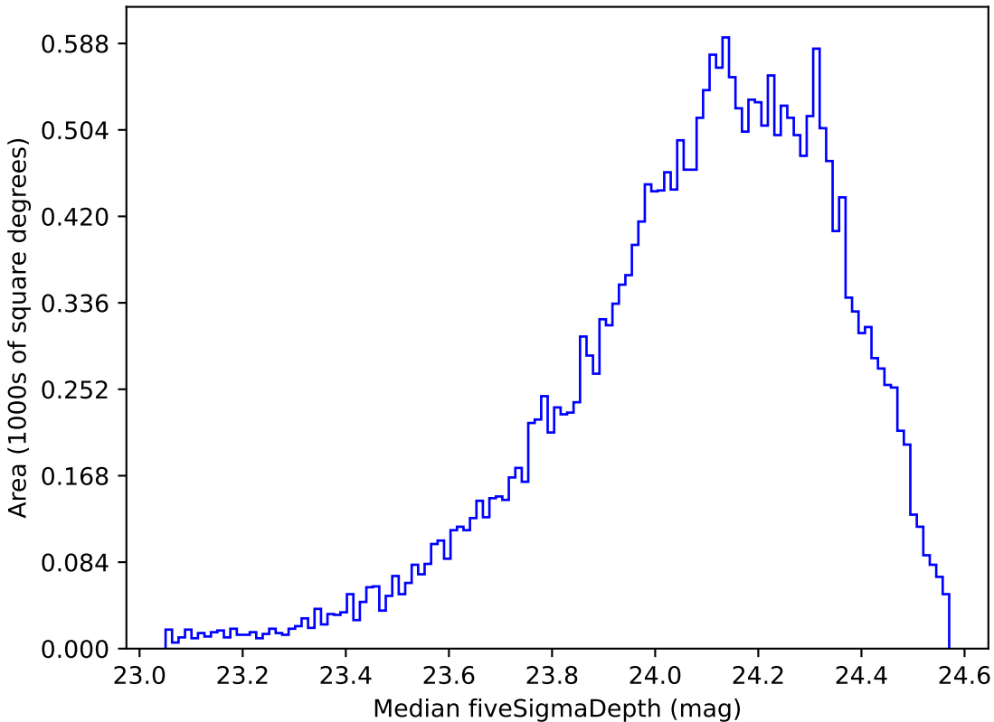
noroll_mjdp60_v3.4_10yrs Yr 1 r band: Median fiveSigmaDepth
