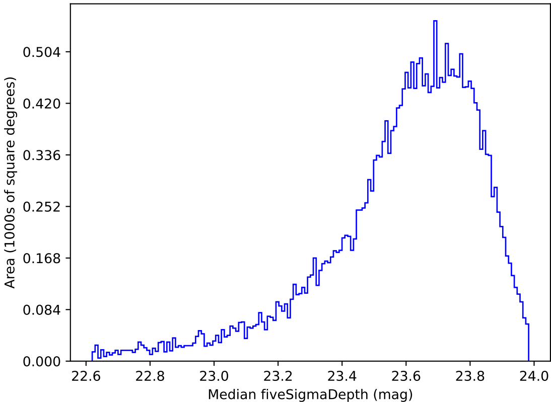
noroll_mjdp60_v3.4_10yrs Yr 1 i band: Median fiveSigmaDepth
