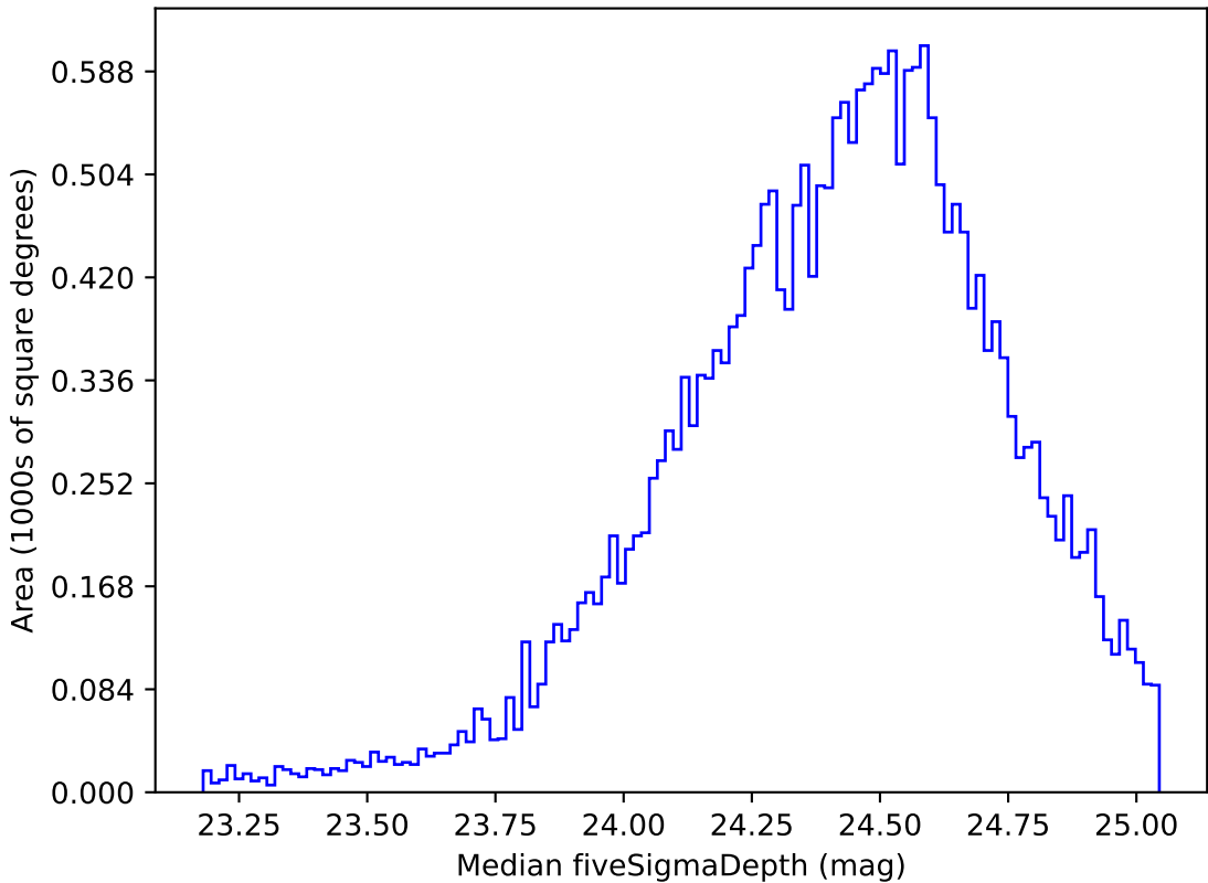
noroll_mjdp60_v3.4_10yrs Yr 1 g band: Median fiveSigmaDepth
