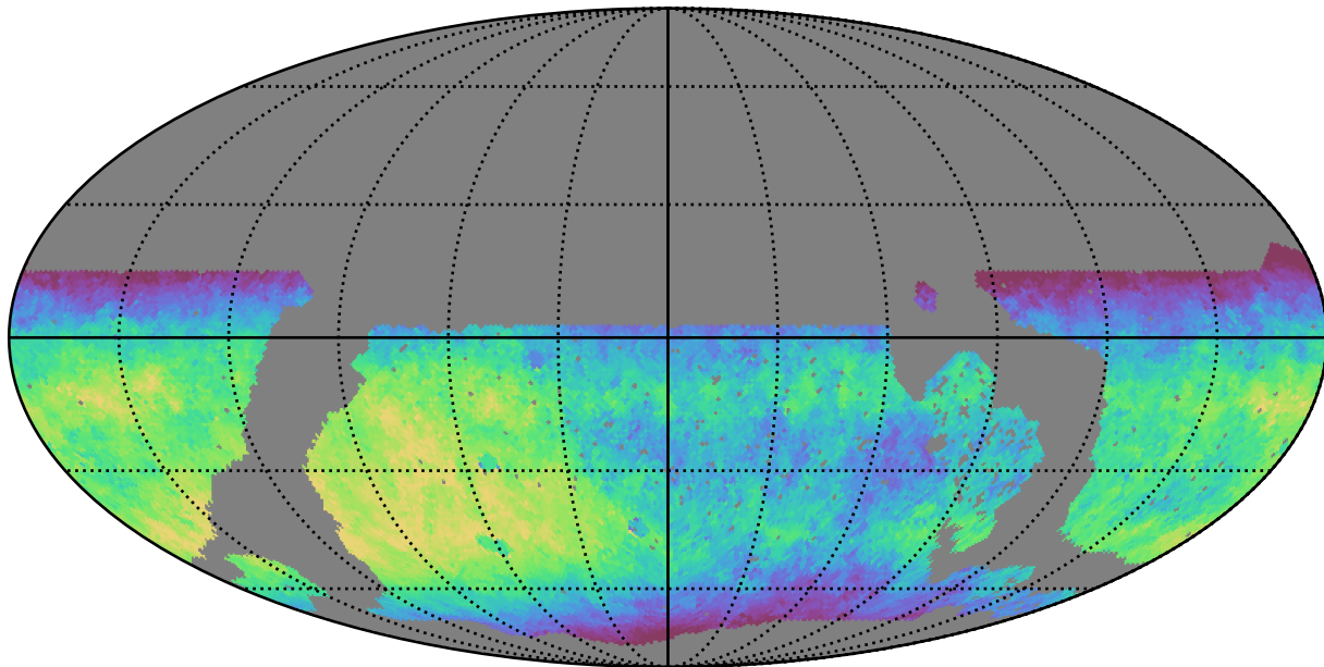
noroll_mjdp60_v3.4_10yrs WFD z band: Median fiveSigmaDepth
