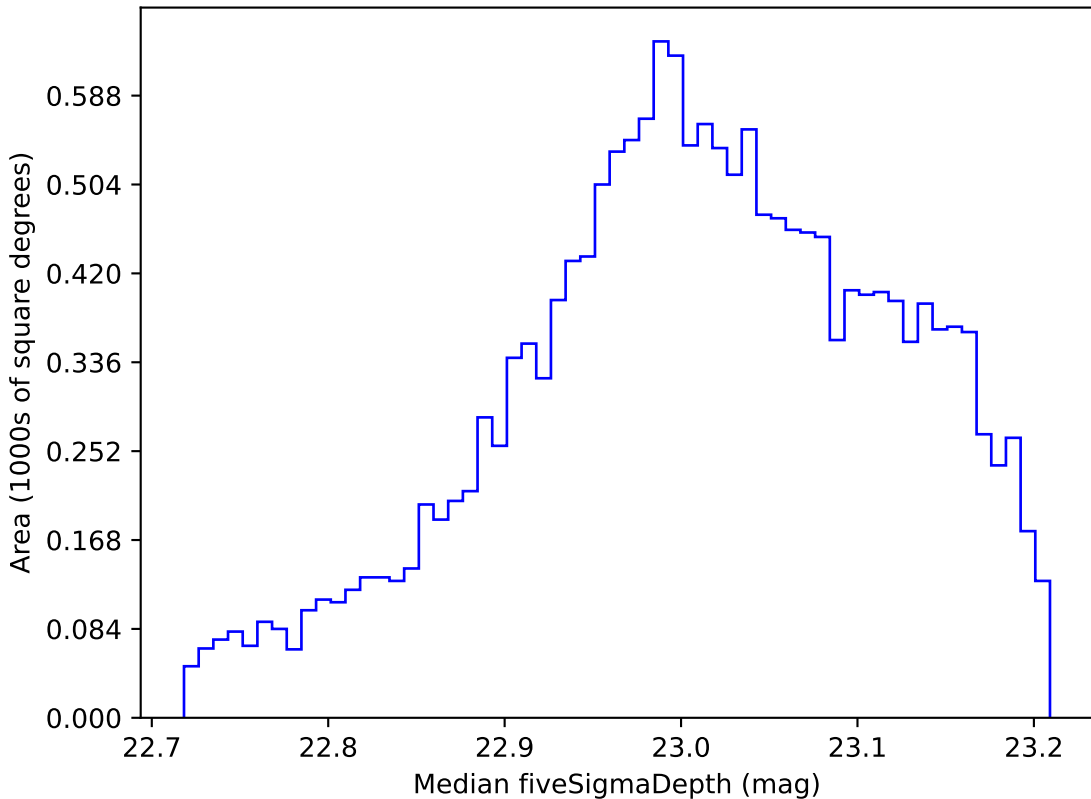
noroll_mjdp60_v3.4_10yrs WFD z band: Median fiveSigmaDepth
