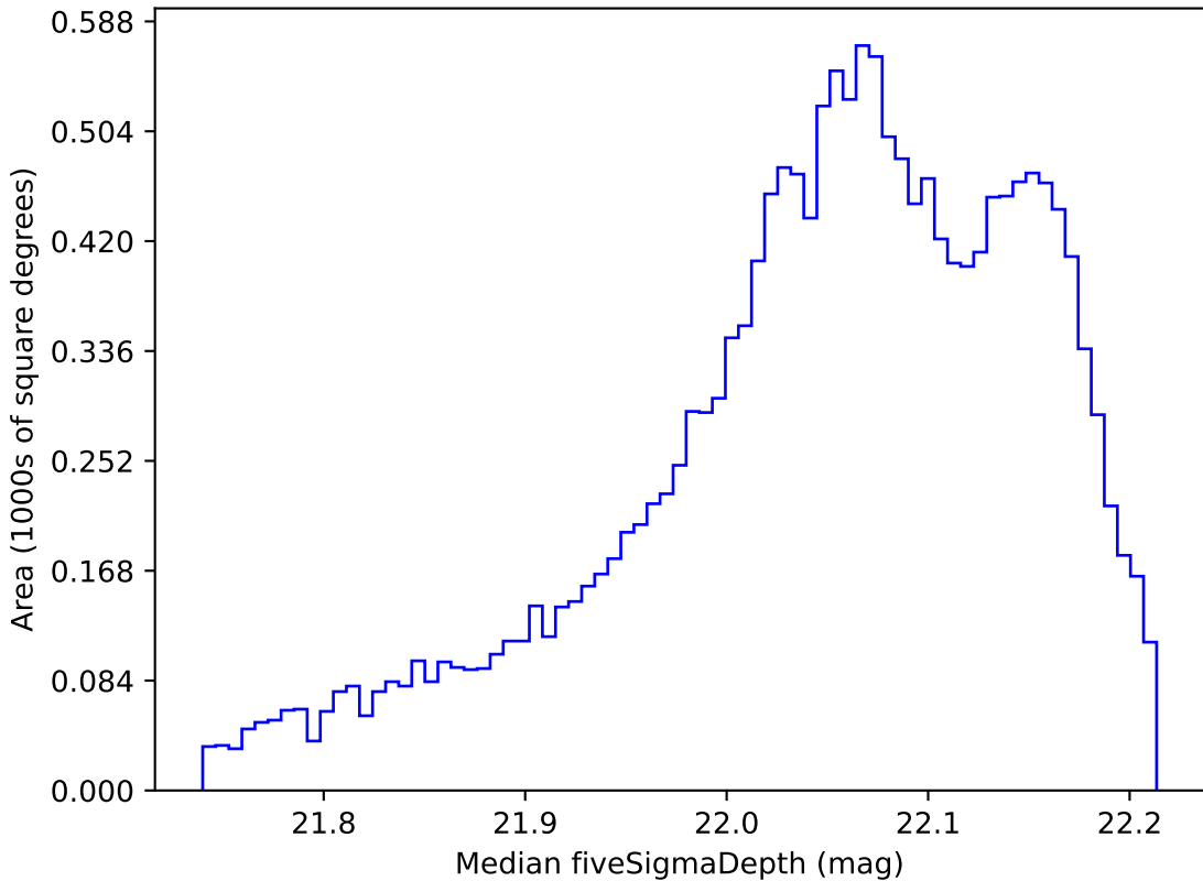
noroll_mjdp60_v3.4_10yrs WFD y band: Median fiveSigmaDepth
