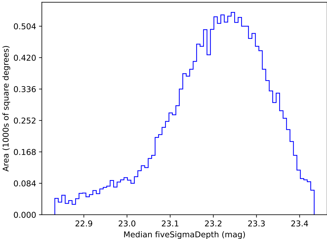
noroll_mjdp60_v3.4_10yrs WFD u band: Median fiveSigmaDepth
