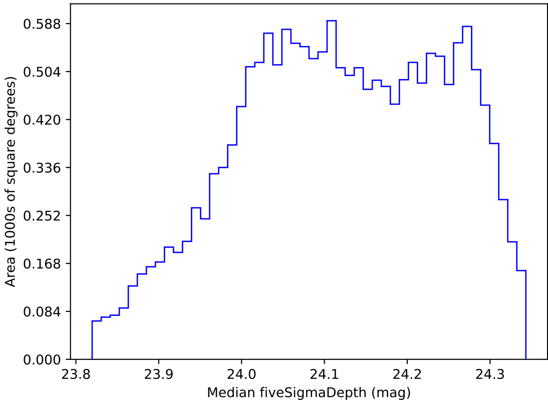
noroll_mjdp60_v3.4_10yrs WFD r band: Median fiveSigmaDepth
