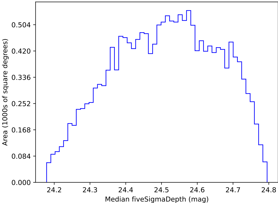
noroll_mjdp60_v3.4_10yrs WFD g band: Median fiveSigmaDepth
