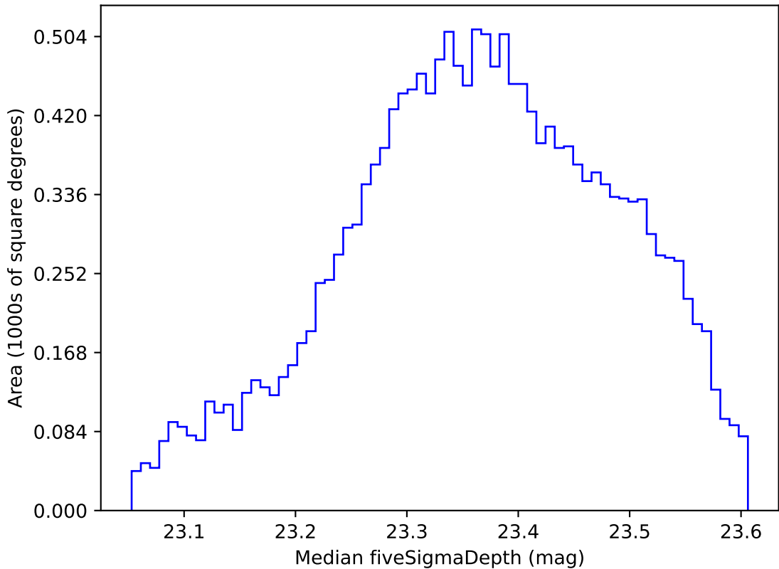
noroll_mjdp60_v3.4_10yrs WFD all bands: Median fiveSigmaDepth
