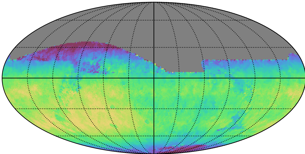
noroll_mjdp60_v3.4_10yrs All sky z band: Median fiveSigmaDepth
