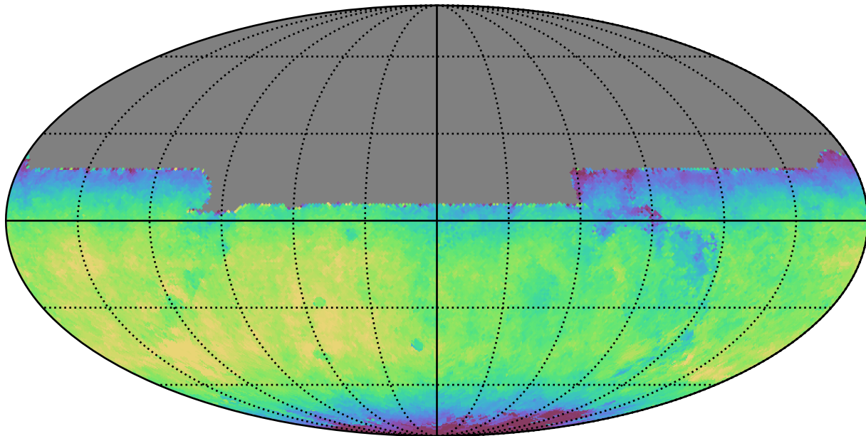
noroll_mjdp60_v3.4_10yrs All sky y band: Median fiveSigmaDepth
